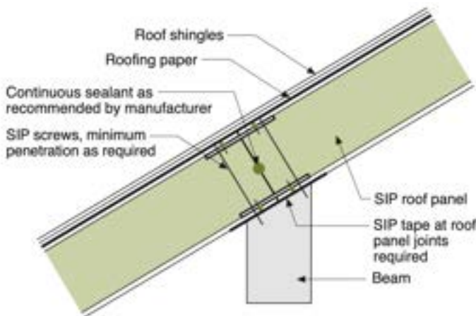
DETAIL 1.5: SIP ROOF - BOX/BLOCK SPLINE JOINT
