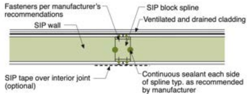
DETAIL 1.6: SIP WALL - BOX/BLOCK SPLINE JOINT
