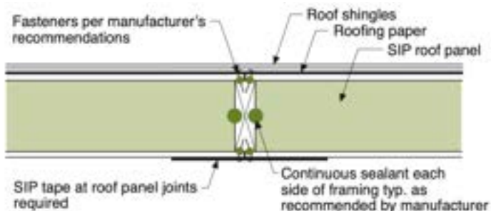
DETAIL 1.2: SIP ROOF - DIMENSIONAL LUMBER SINGLE SPLINE JOINT
