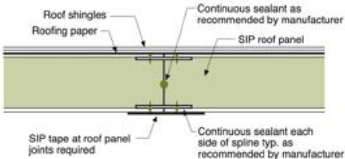
DETAIL 1.3: SIP ROOF - SURFACE SPLINE JOINT
