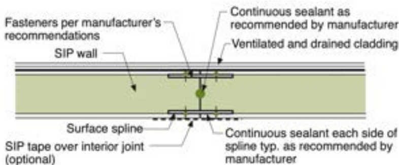
DETAIL 1.7: SIP WALL - SURFACE SPLINE JOINT
