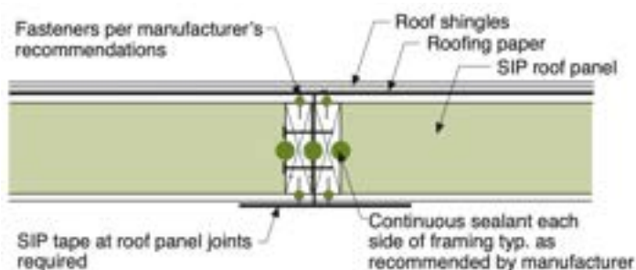
DETAIL 1.1: SIP ROOF - DIMENSIONAL LUMBER DOUBLE SPLINE JOINT
