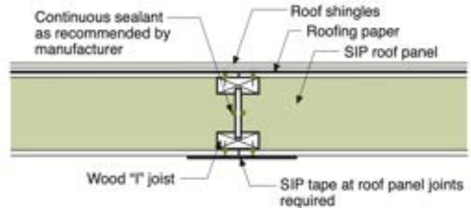
DETAIL 1.4: SIP ROOF - I-JOIST SPLINE JOINT
