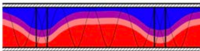
FIGURE 1.3: TRADITIONAL STICK FRAMED WALL CROSS- SECTION WITH FIBERGLASS*
