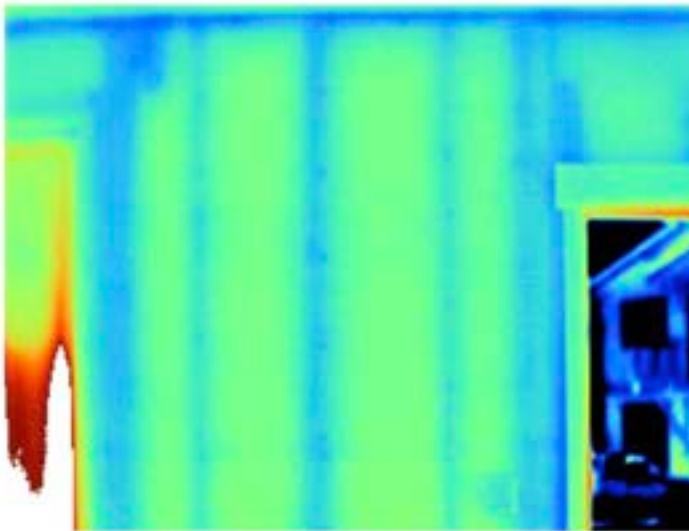
IMAGE 1.7: MINNESOTA SIP HOUSE (THERMAL)
